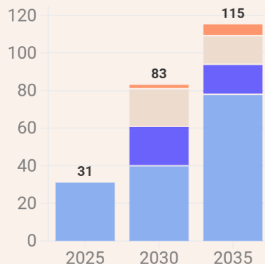
Cell production (GWh)
